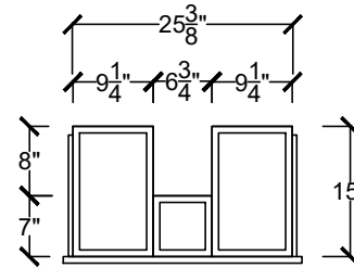
DRAWER BOX DETAIL
